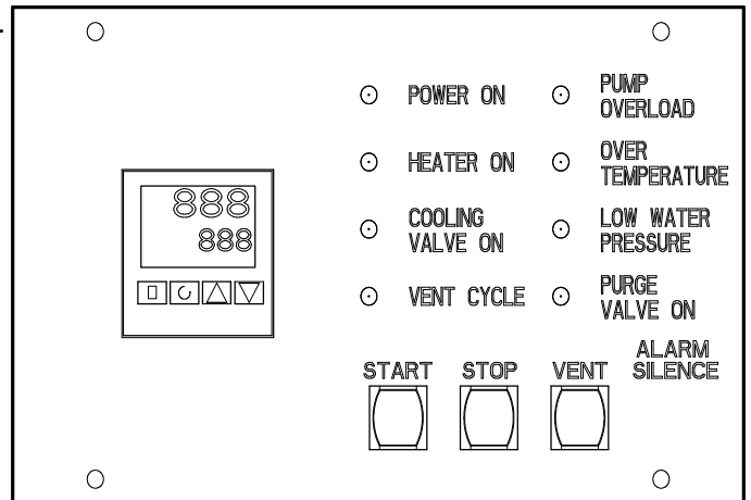
Standard Controller
