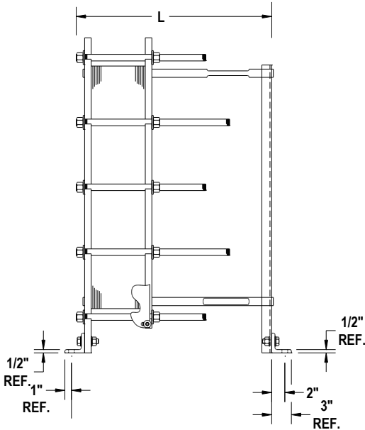
Plate & Frame Heat Exchanger Side View
